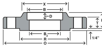
SOCKET WELD
